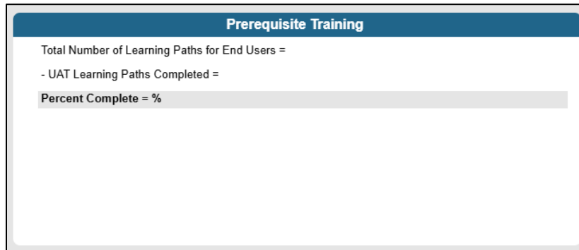
Figure 26: Prerequisite Training
