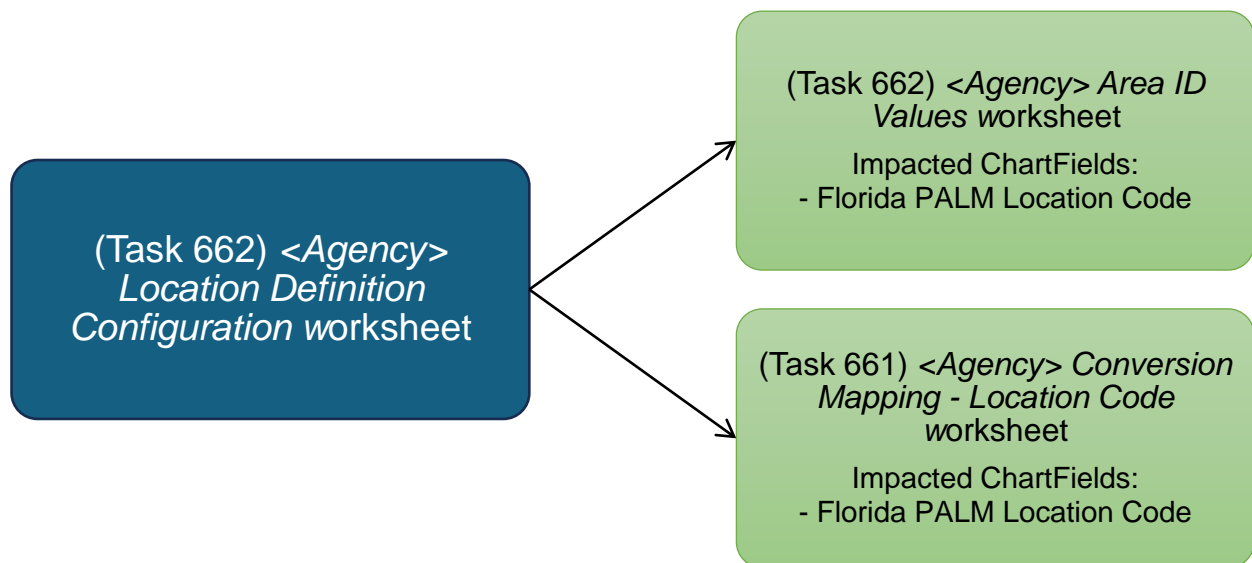
Figure 3: Cross-worksheet Connections for Location Definition
