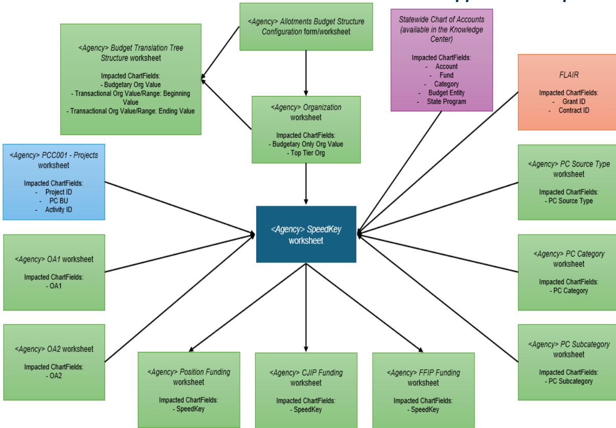
Figure 4: Cross-worksheet Connections for SpeedKey
