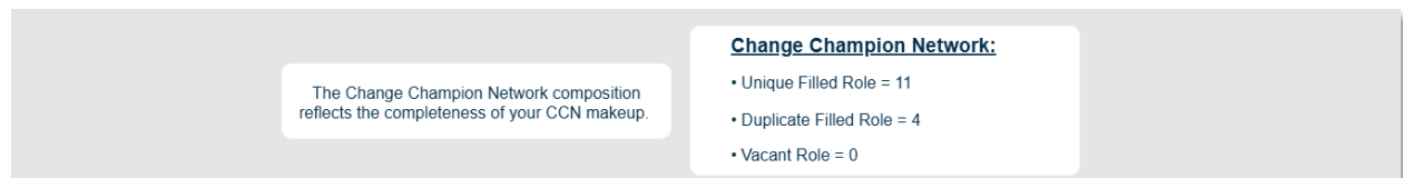
Figure 11: CCN Composition
